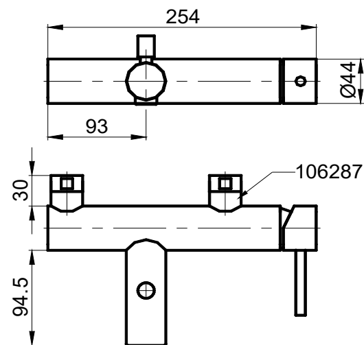
sketches and dimension with 106287 and 106286 schizzi e dimensioni con 106287 e 106286
